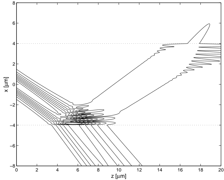
Figure 4: Contour plot of the magnitude of the solution in a horizontally stratified medium
