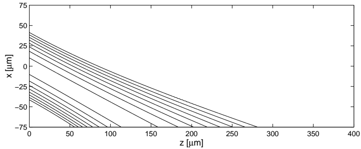
Figure 2: As in the preceeding figure, except for 2561 grid points
