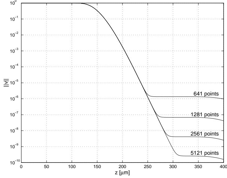
Figure 3: The L^2 -norm in the interior domain for 641, 1281, 2561, and 5121 transverse grid points
